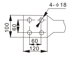
GN22-12C/2500~3150 Connection terminal
